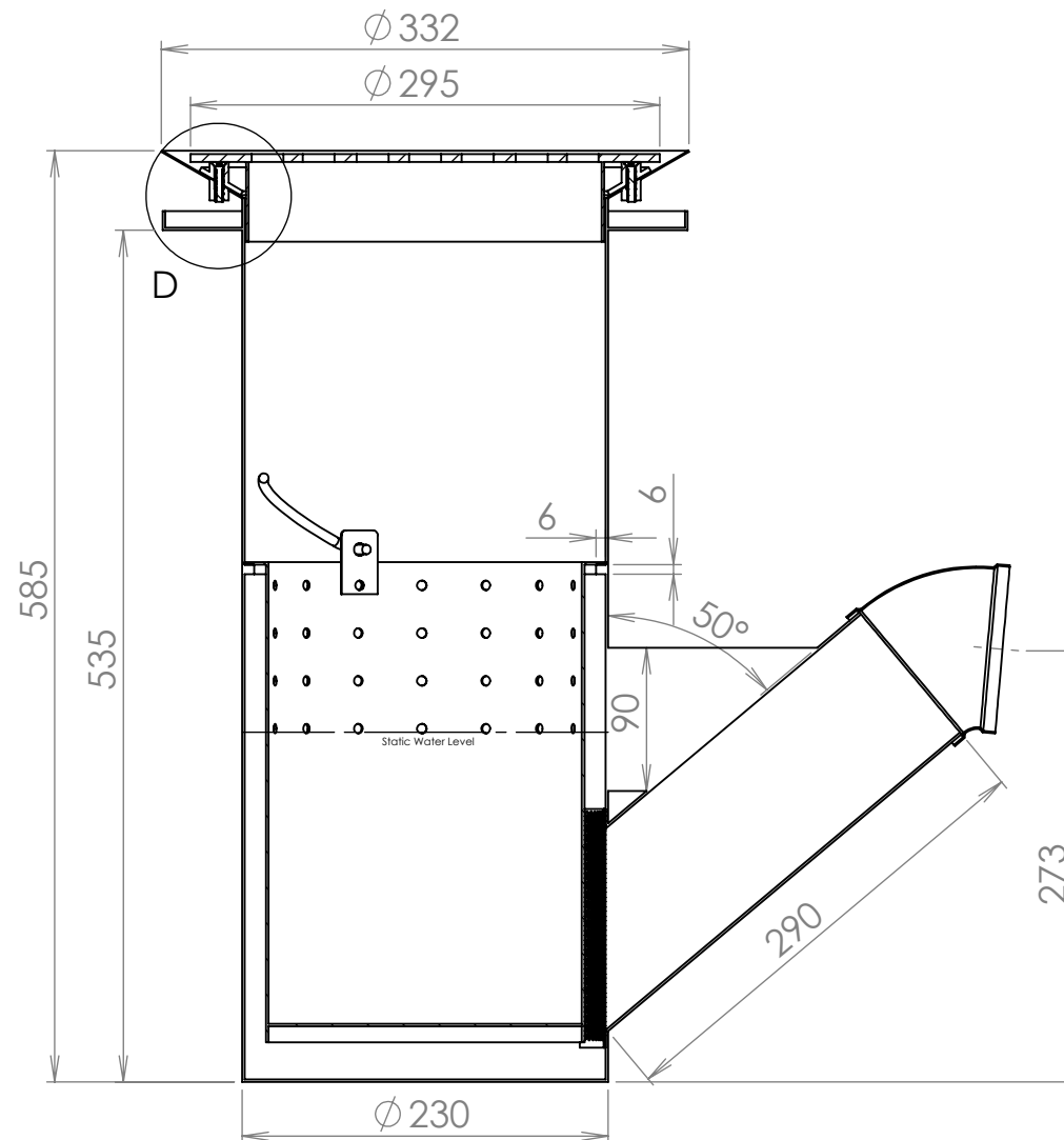
SECTION C-C
