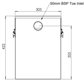
MODEL OSPC Front Elevation
