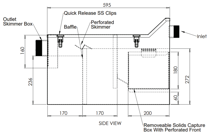
MODEL OSPC Side Elevation
